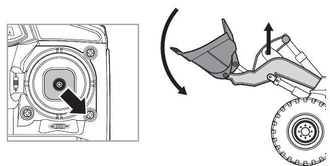
Arm Rising while Bucket Downdipping
