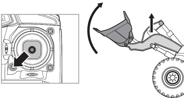
Arm Rising while Bucket Updipping
