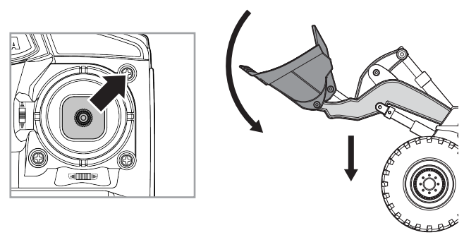
Arm Lowering while Bucket Downdipping
